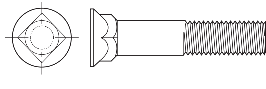
BOULONS DE CHARRUE, TÊTE NO. 3 NO. 3 HEAD PLOW BOLTS
