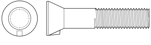
BOULONS DE CHARRUE, TÊTE NO. 7 NO. 7 HEAD PLOW BOLTS
